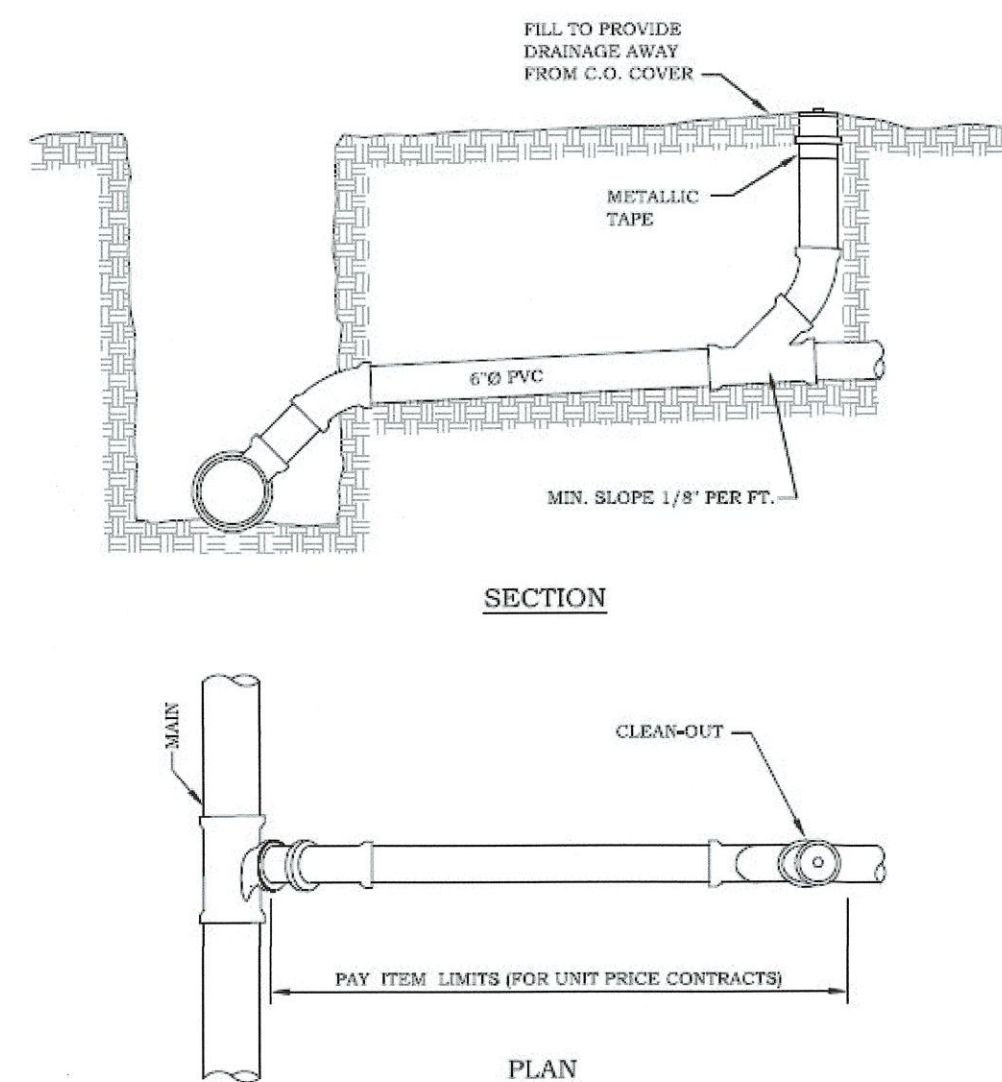
SEWER SERVICE LINE DETAIL NTS
